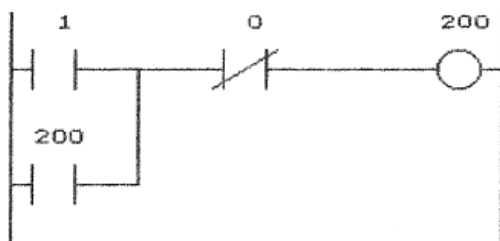
Ladder diagram
